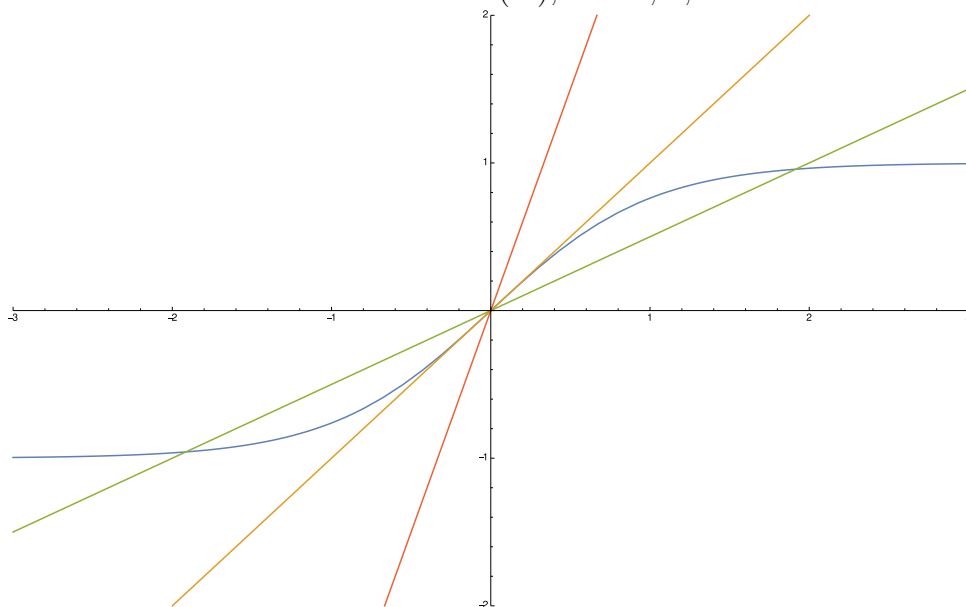
Рис. 1: T\tilde{m} = \tanh(\tilde{m}) , T = 3; 1; 0.5
