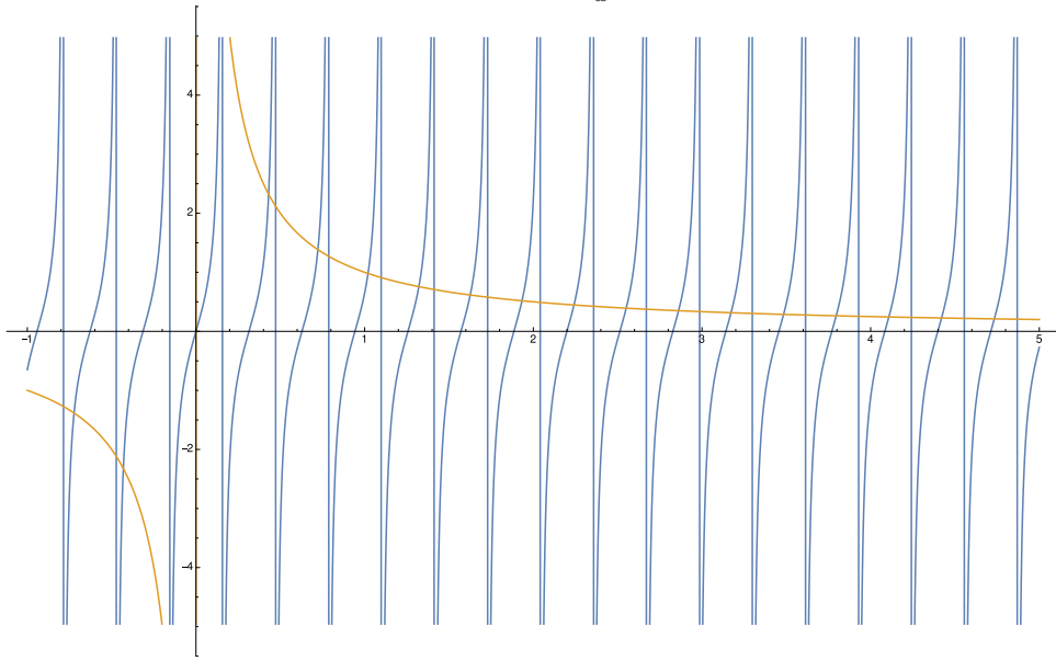
Рис. 3: \tan Ax = \frac{1}{x} , A = 10
